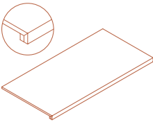
Degrau "L" Step tread "L" Nez de marche "L" Stufenplatte "L" 30x100 Ret. LP-6635 30x100 Ret. AS LP-6635
